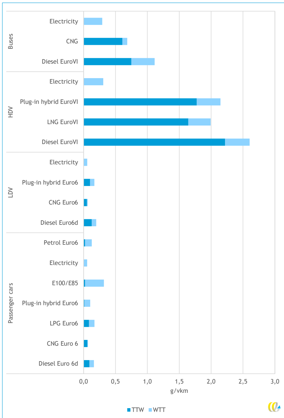
Figure 1 - Emission factors of NO x (tank-to-wheel and well-to-tank) for different vehicle technologies
