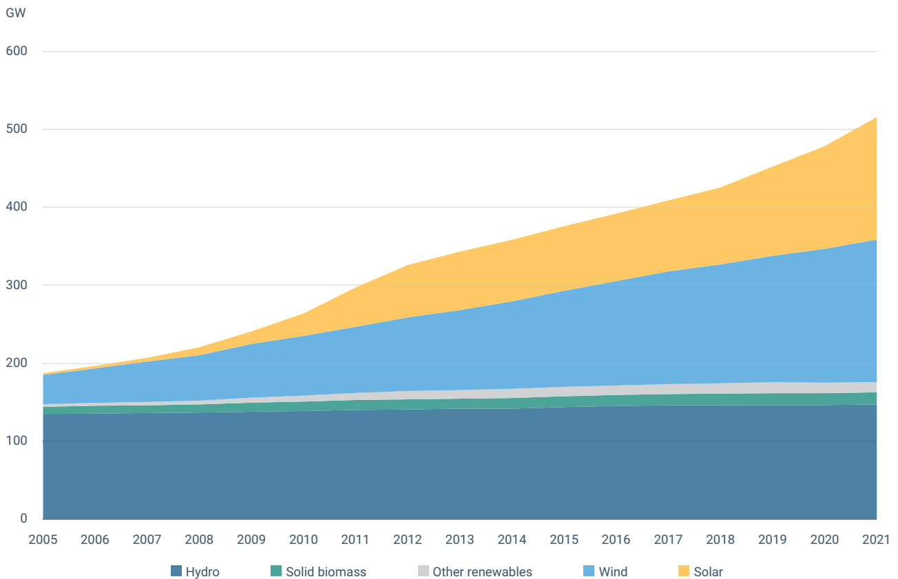
Figure 1.9 RES-E capacities in gigawatts
