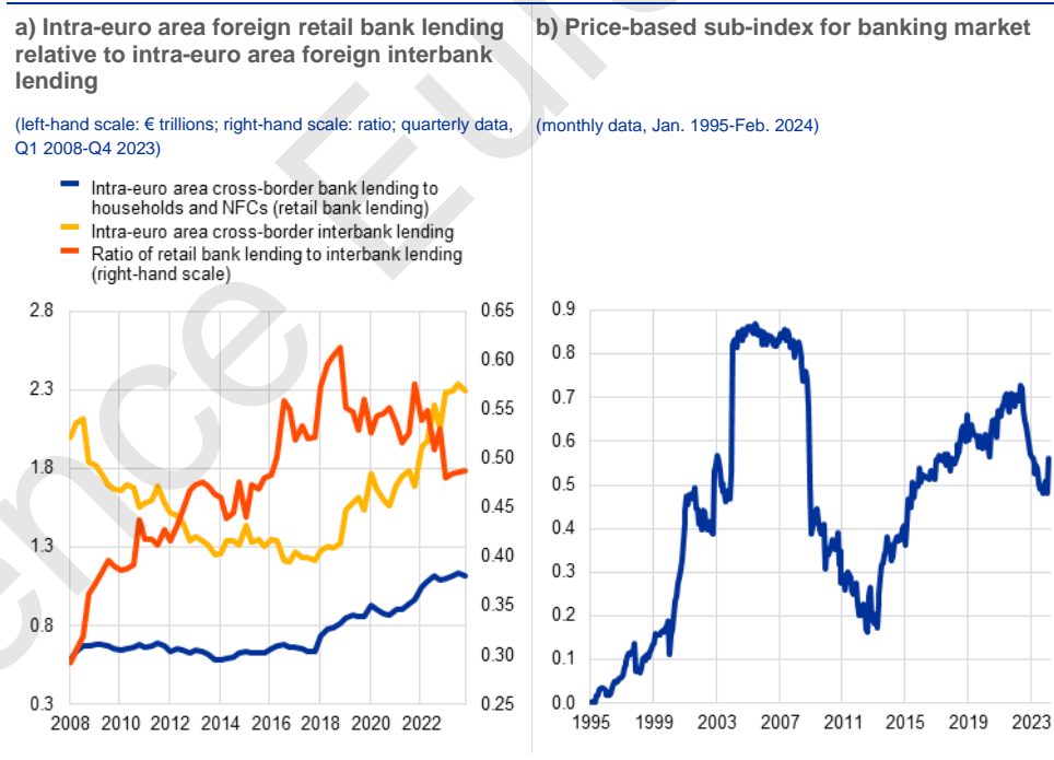
Chart 14 Euro area banking market integration in quality and price terms
