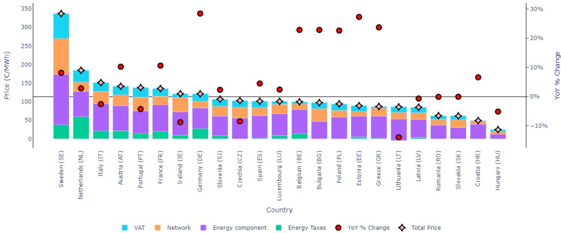
Figure 42 – Year-on-year change in gas price components in the European capitals comparing Q1 2025 with Q1 2024
