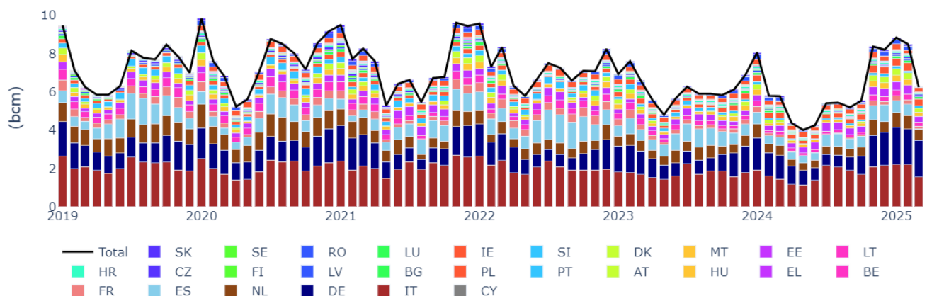
Figure 11 - Monthly gas usage in power generation
