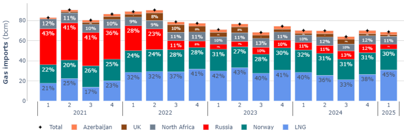
Figure 14 – Quarterly share of gas imports within the total, combining both pipeline and LNG imports
